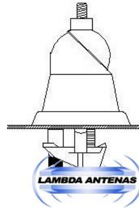
CM-70G Mounting Base
